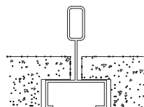
15/16" Slot Ceiling
