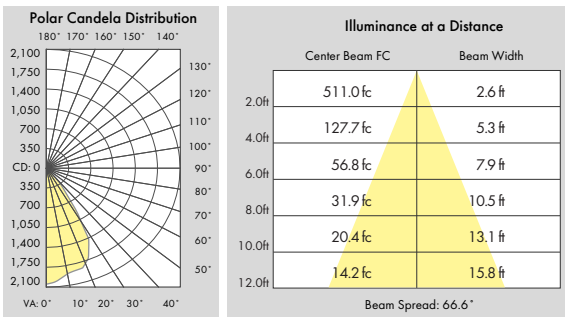
VLED-ARFK9-30-830+LEDT-R94]
