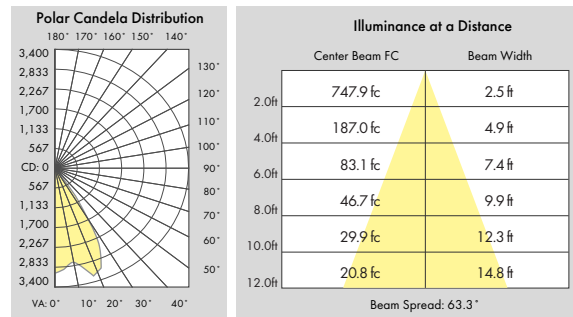
[VLED-ARFK9-45-830+LEDT-R94]
