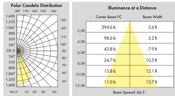
V[LED-ARFK9-23-830-W+LEDT-R94]
