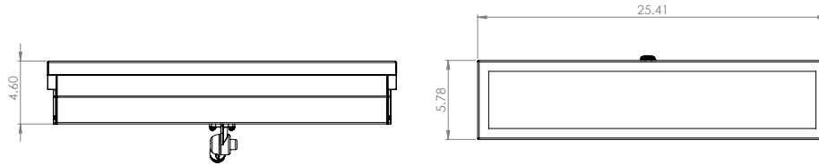
Dimensions shown for 24" Unit only.
