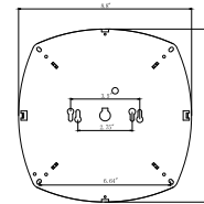
8.5" Round Light Engine
