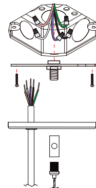
Various "Hard Ceilings" (Mount to J-box)
