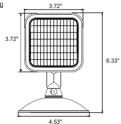
VE-RH-1(WH)
