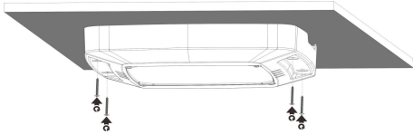
Surface mount
